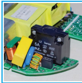
Smart fuse: reset once overload 5A
