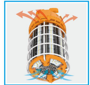
Air convection design between up and down of the lamp, promoting the heat dissipation function so that could ensure the lamp lifespan.
